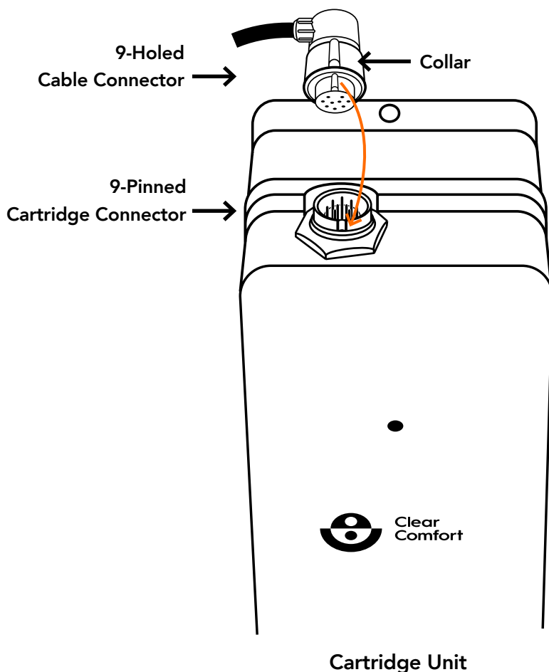
Figure 3: Cartridge Connection
