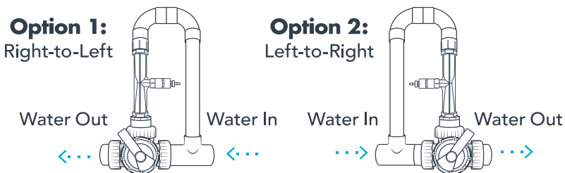
Figure 6: Manifold Orientation
