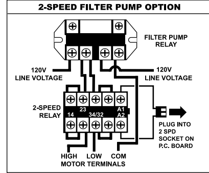
WIRING DIAGRAM IntelliTouch Models 15+3 • 17+3 • 19+3
