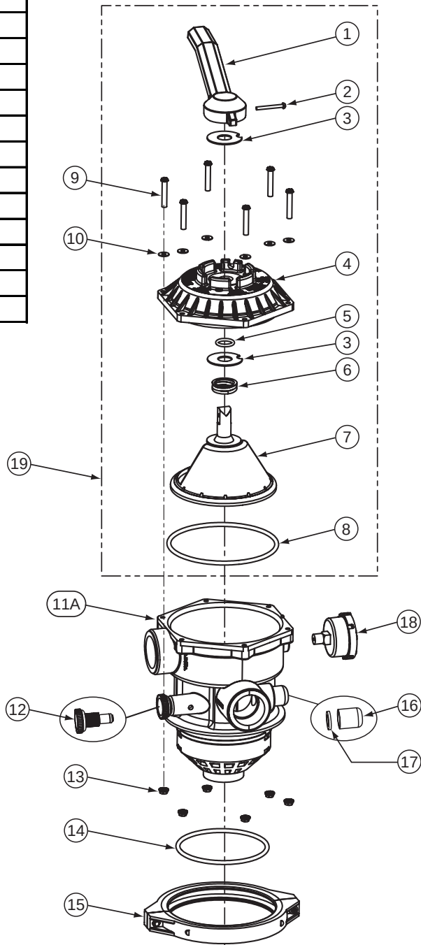
CLAMP STYLE VALVE
